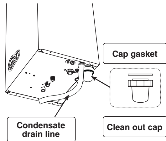
Figure 3 Boiler condensate trap
