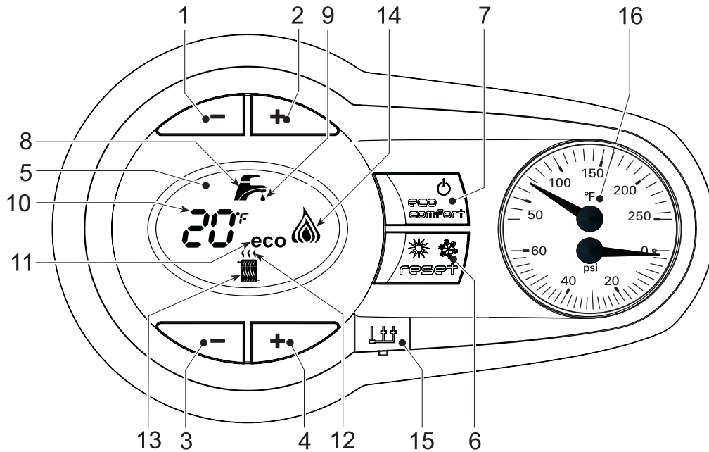
Figure 6 Control module
